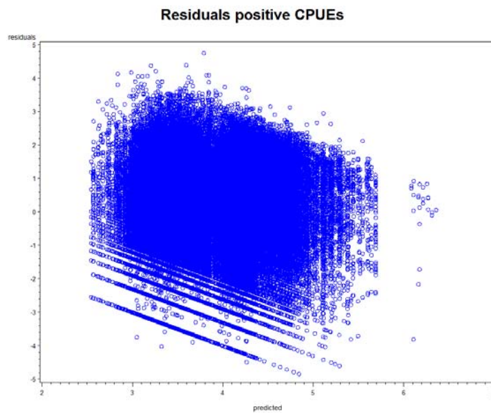
Figure 4. Plot of the predicted CPUE and residual from positive catch rate model.
